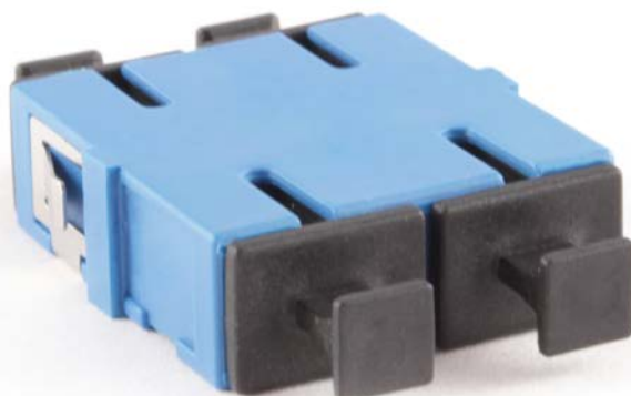
P/N: 48SMTSCDFL SC/SC UPC duplex blue adapter SM flangeless Suitable for OS1/OS2
