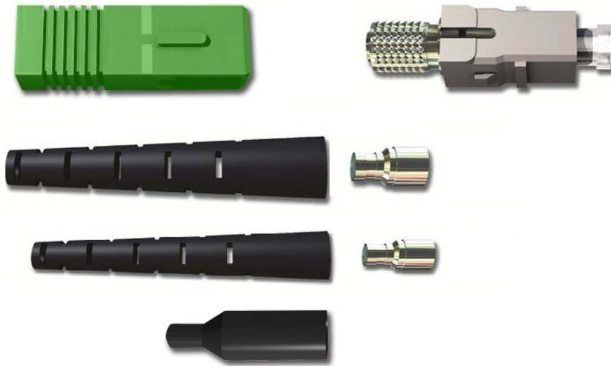
P/N: 48SMCSCAS SC APC 8° simplex connector, suitable for OS1, OS2
