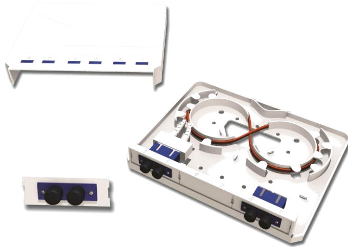
P/N: 48BMOP3P (shown loaded)
